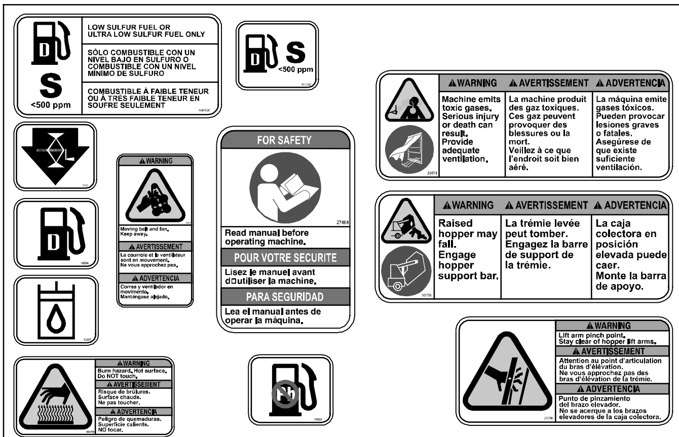
Fig. 80 - Label Group
