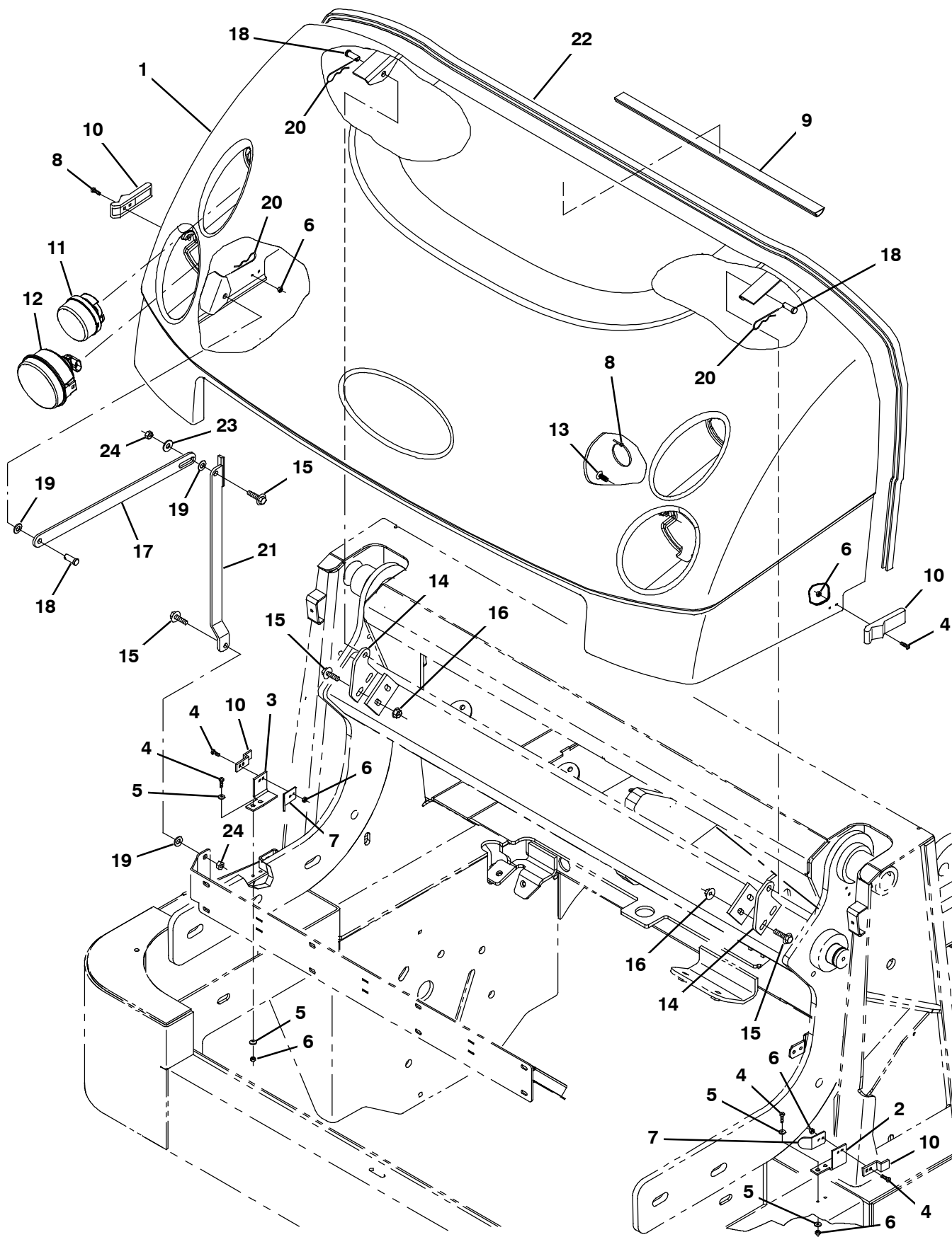
Fig. 43 - Hopper Cover Group (000000-002099)
